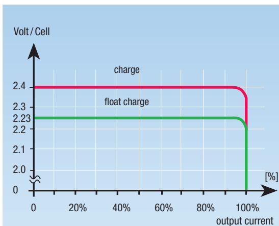
Fig 3: Charging characteristic for lead-acid batteries in accordance with DIN 41773
